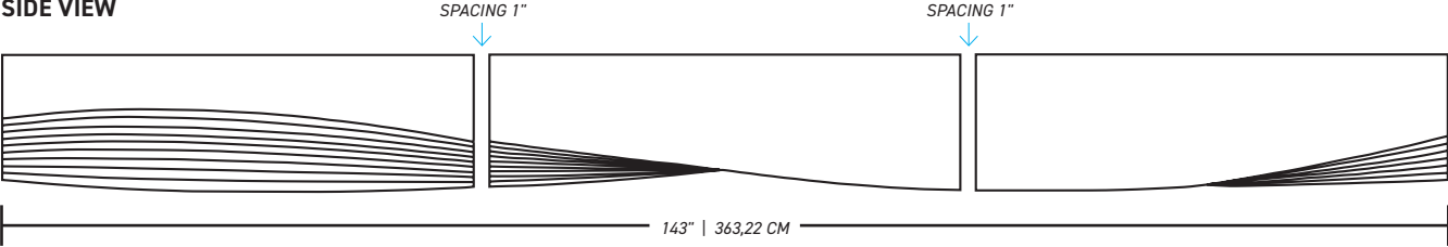
SIDE VIEW
